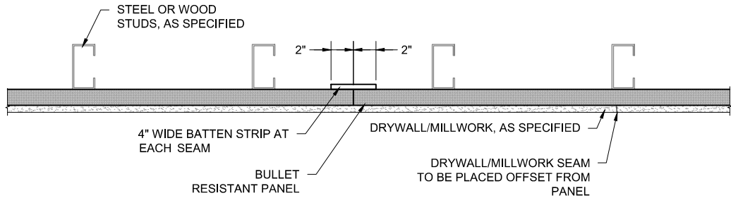
PLAN VIEW
