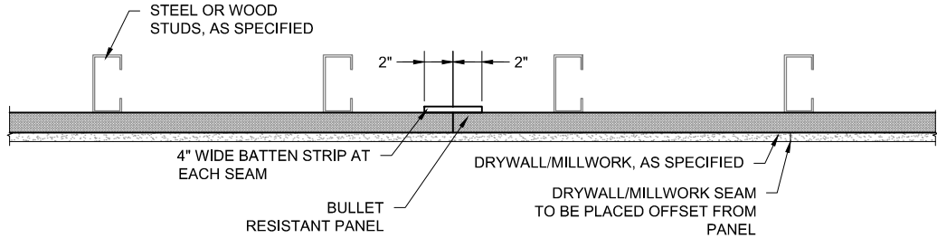
PLAN VIEW
