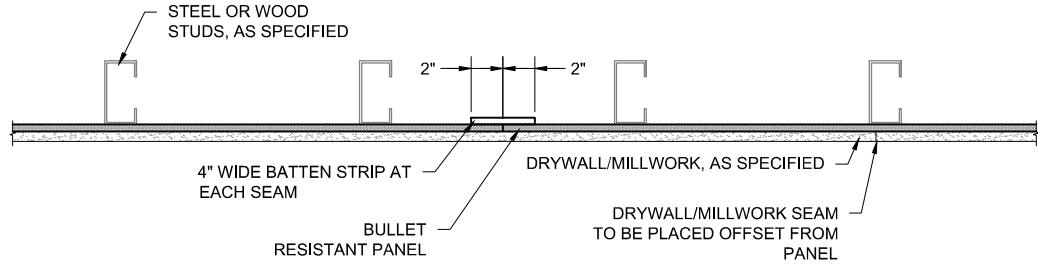
PLAN VIEW
