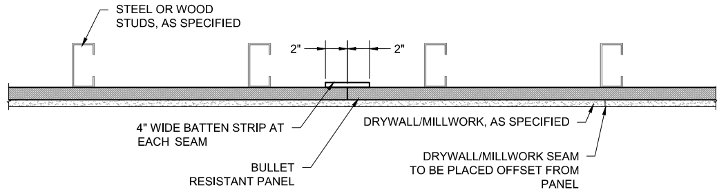
PLAN VIEW
