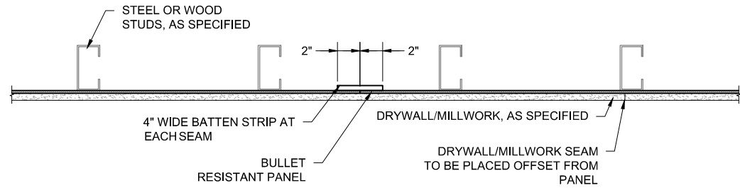
PLAN VIEW
