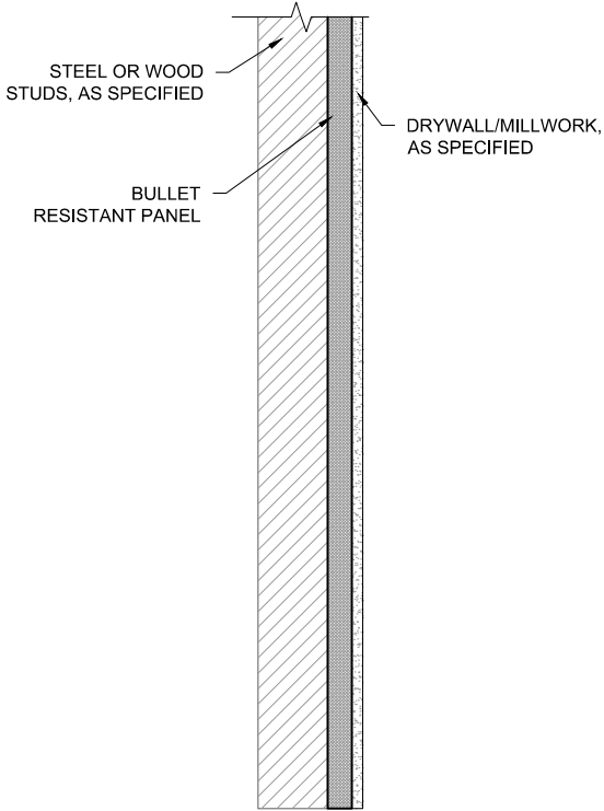
SECTION VIEW
