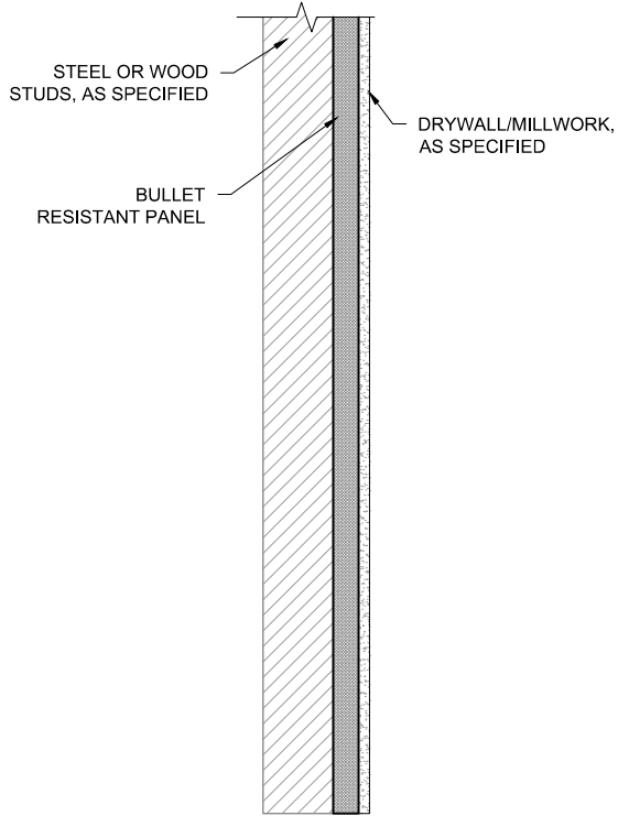
SECTION VIEW
