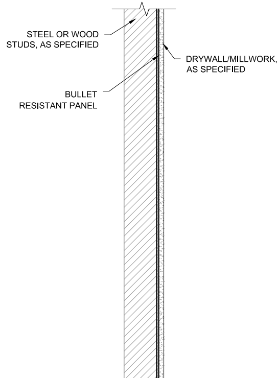
SECTION VIEW
