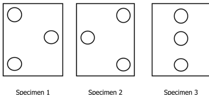
FIG. 2 Impact Locations for Small Missile Test (Each Type of Infill)
